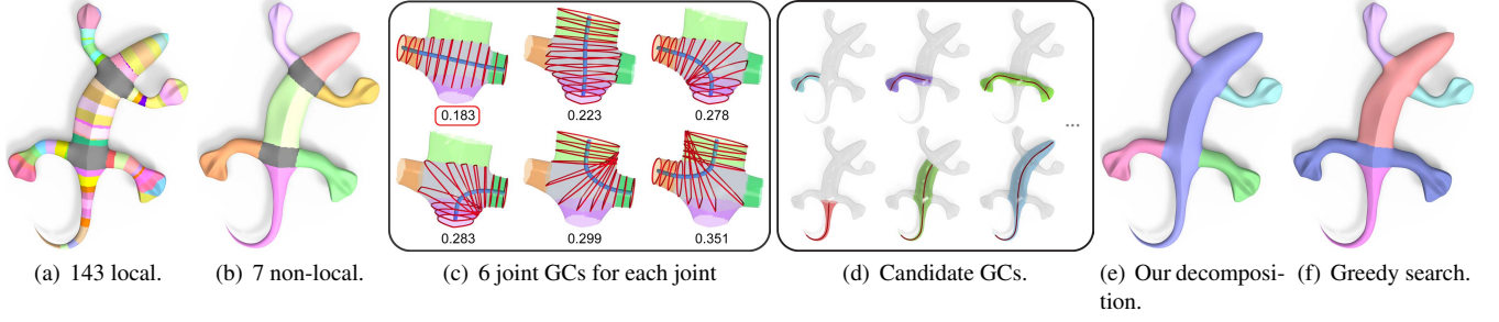
Figure 7: Merge 143 local GCs (a) of a Gecko model into 7 non-local GCs (b) using the criterion defined in (5). Note that the two X-shaped joints (dark gray) are not covered in both (a) and (b). To cover them, we set up six different ways of connecting adjacent GCs (c). A set of candidate GCs (d) are then computed using the 7 non-local GCs and 12 joint GCs to find the global optimal exact cover, i.e., our decomposition (e). In comparison, a greedy search would pick the first joint GC in (c) out of the 6 choices, resulting a suboptimal decomposition (f).
