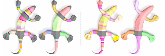
Figure 10: Impact of parameter \tau . Left: setting \tau = 0.12 leads to 118 local GCs, which are merged into 10 non-local GCs. Right: with \tau = 0.25 , 196 local and 6 non-local GCs are formed. The results under \tau = 0.15 are shown in Figure 7. Although having different numbers of local GCs and non-local GCs, the final decompositions under all three \tau values are the same.
