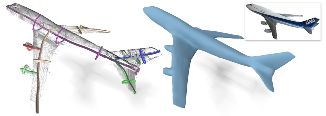
Figure 13: The real airplane object (inset) contains non-cylindrical parts and the input point cloud (left) is incomplete. Yet, our approach successfully reconstructs a 3D model (right) that respects the raw scan and is close to the real object. Different branch paths processed by morfit are shown in different colors.
