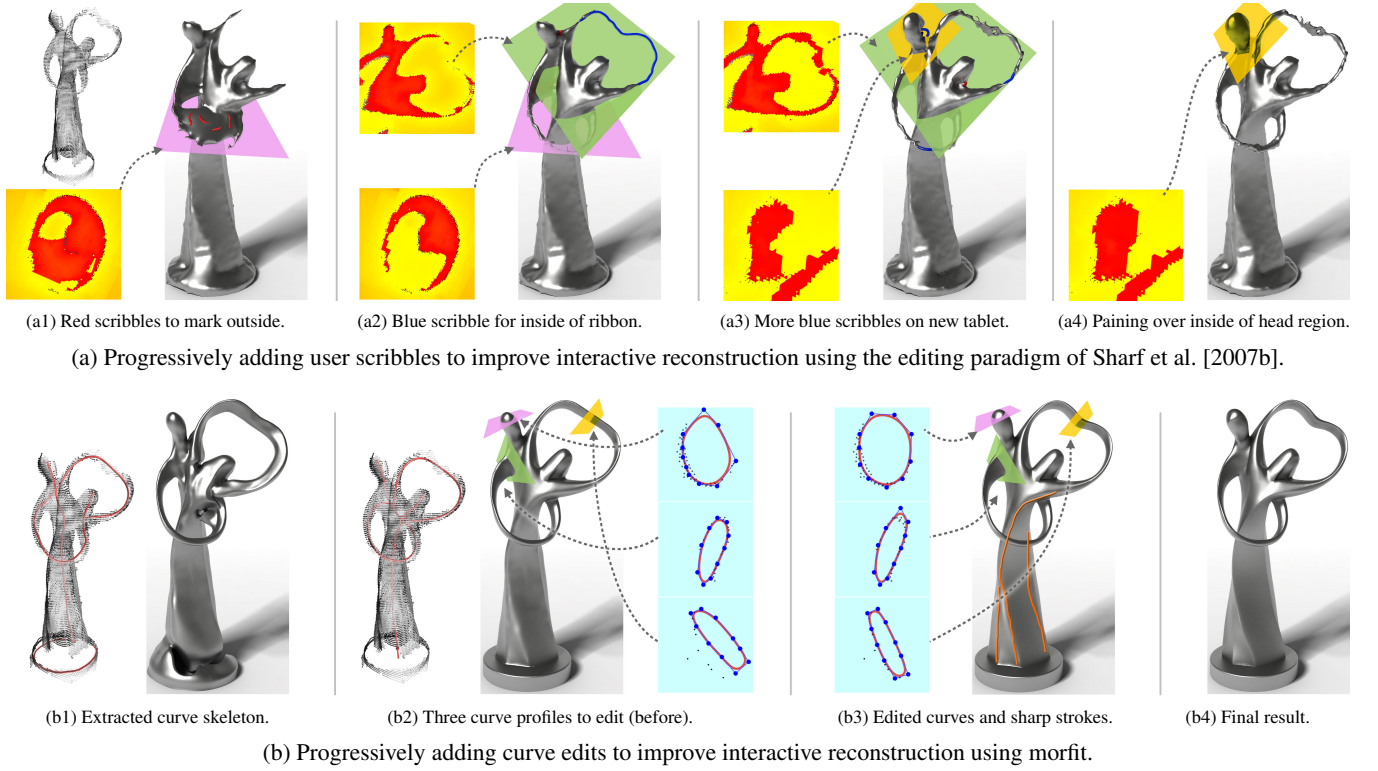
Figure 14: Comparing morfit (b) with the state-of-the-art interactive surface reconstruction method by Sharf et al. [2007b] (a) in terms of how user interactions progressively improve the reconstruction. To accurately reconstruct over regions with significant missing data, Sharf et al.’s method requires proper placement of 2D tablets (colored profile planes in top row), on which topology information is specified (red \rightarrow inside, yellow \rightarrow outside). Here, these tablets were placed with great care for achieving better results. However, it is still hard to fully cover regions with significant missing data, e.g., near a thin structure where data is almost entirely missing (a2 and a3). Inside of a tablet, the user needs to correct the wrong topology or geometry by “painting” over wrong inside regions using red scribbles (a1) and wrong outside regions using blue scribbles (a2). This process is quite tedious and prone to imprecisions, e.g., due to slightly misplaced tablets, leading to rough and low-quality reconstruction results (a3 and a4). In contrast, morfit relies on user interaction on 1D curves where 6 skeleton edits, 3 profile curve edits (see before and after shown in (b2) and (b3)), as well as 3 sweep path strokes and 3 sharpening strokes, provide the fine-grained topology and geometry controls enough to obtain a faithful and quality reconstruction (b4).
